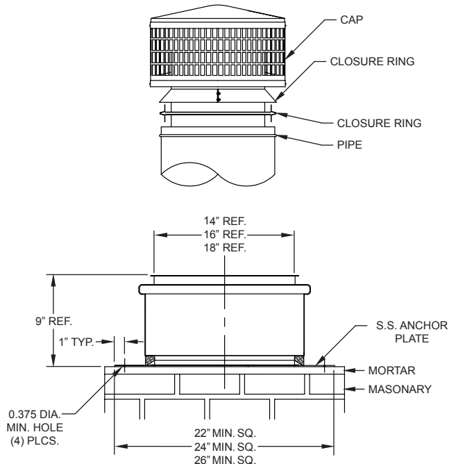
FIG. 15b 14TG, 15TG, AND 18TG ANCHOR PLATE
