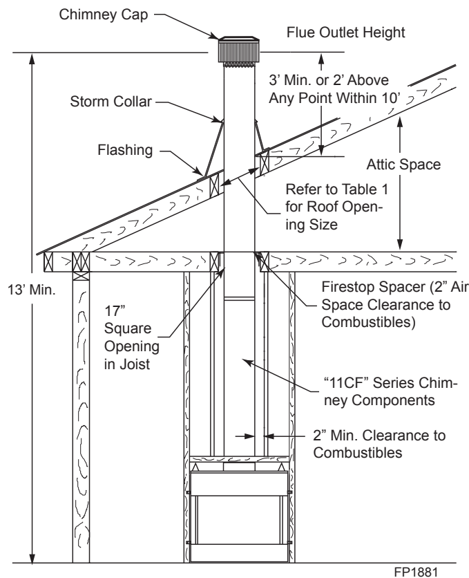
Figure 5 Single Story Installation with Attic Space
