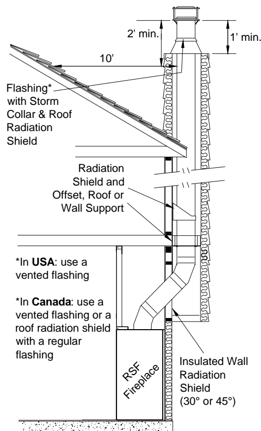
Figure 11 Offset Chimney Through a Wall Example
